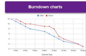
Burndown charts
